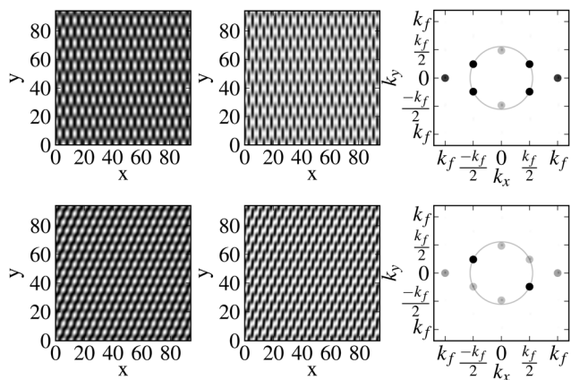
Fig. 9 Resonant 2:1 rectangular pattern (top row) and oblique pattern (bottom row) in the LE model. The left and middle frames show the v and u -field patterns in the (x, y) plane. The right frames show the corresponding spatial Fourier transform of u in the (k_x, k_y) plane. The shading of the circles in the Fourier plane indicates the strength of the modes (darker is higher). Note the asymmetry in the strength of the two oblique modes for the rectangular pattern and the presence of the forcing wave-vector in the rectangular pattern. Parameters: a = 12 , d = 1 , \sigma = 50 , w_0 = 0 , \gamma = 0.6 , k_f = 1.8k_T , and b = 0.38 (rectangular pattern) and b = 0.35 (oblique pattern).
